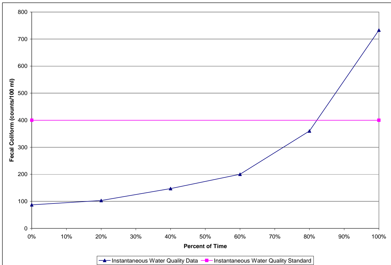
Figure 5. 10% Test Curve for Station A0210005, Summer 2008
